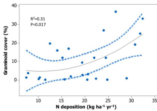
Upland heath: graminoid cover
