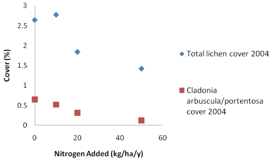
Figure 12: Response of lichens to nitrogen addition in montane heath at Culardocho in the Cairngorms (Britton & Fisher, 2007). Background N deposition circa 10 \text{ kg N ha}^{-1} \text{ yr}^{-1} .
