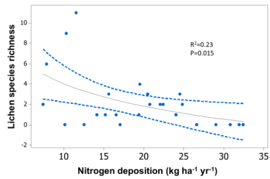
Upland heath: lichen species richness
