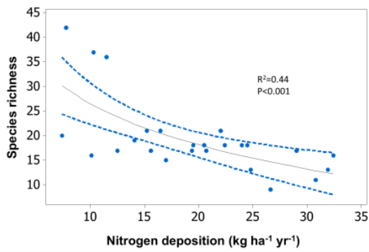
Upland heath: total species richness
